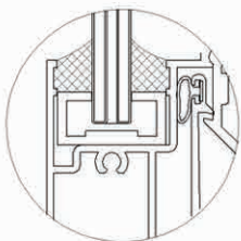
5/16" Laminated
