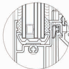
1 1/16" or 3/4" Lami/Insulated
