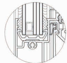
1 1/16" or 3/4" Lami/Insulated
